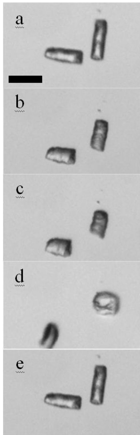
Figure 4. Contraction of isolated nematic main-chain LCE pillars heated up to the isotropic (a–d), then cooled back to room temperature (e). Scale bare is 100 \mu\text{m} . A movie in AVI format shows this in motion.
