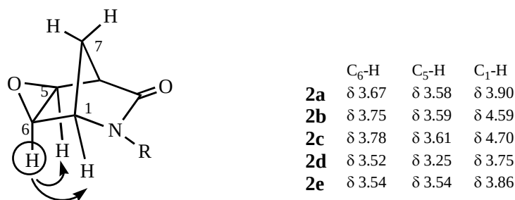
NOE correlations of 2
