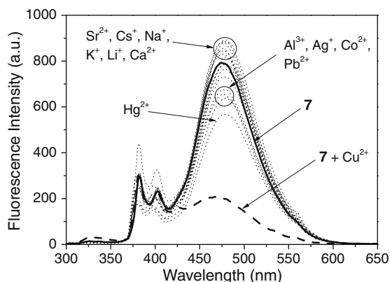
Figure 2. Fluorescence spectra of 7 (6.0 \mu M) upon addition of various cations (100.0 equiv) in \text{CH}_3\text{CN}/\text{CHCl}_3 (40:1, v/v) with an excitation wavelength at 280 nm.
