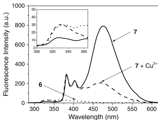
Figure 4. Fluorescence spectra of 6 and 7 (6.0 \mu M, respectively) in the presence of \text{Cu}^{2+} ion (100.0 equiv) in \text{CH}_3\text{CN}/\text{CHCl}_3 (40:1, v/v) with an excitation at 280 nm. Inset: enlarged spectra of 6 and 7 between 300 and 365 nm.
