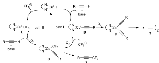
Scheme 1. Plausible Reaction Pathways for Trifluoromethylation
