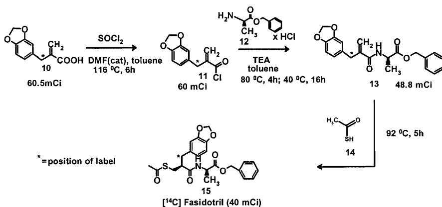
Scheme 3. Completion of the synthesis of [ ^{14}\text{C} ]Fasidotril
