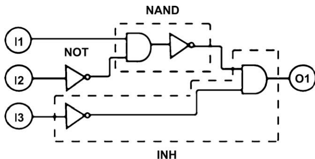
Figure 4. The combinational logic circuits equivalent to the truth table gave in Table 1.
