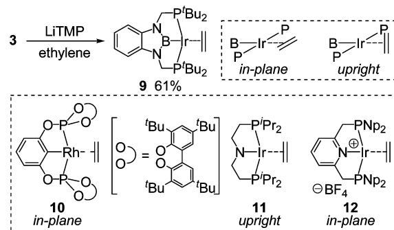
Scheme 4. Synthesis of PBP(ethylene)iridium(I) Complex 9 and Related Compounds 10–12 (TMP = 2,2,6,6-Tetramethylpiperidine, Np = Neopentyl)
