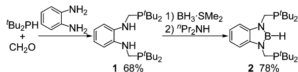
Scheme 1. Synthesis of Hydroborane 2
