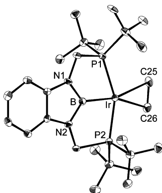
Figure 4. Crystal structure of [PBP](ethylene)iridium(I) complex 8 (50% thermal ellipsoids; hydrogen atoms were omitted for clarity). Selected bond lengths (Å) and angles (deg): Ir–B, 2.048(3); Ir–C(25), 2.205(3); Ir–C(26), 2.208(3); Ir–P(1), 2.3145(9); Ir–P(2), 2.3100(10); C(25)–C(26), 1.393(5); B–N(1), 1.443(4); B–N(2), 1.439(4); C(25)–Ir–C(26), 36.81(12); Ir–C(25)–C(26), 71.74(19); Ir–C(26)–C(25), 71.45(19); P(1)–Ir–P(2), 150.67(3); B–Ir–C(25), 161.92(14); B–Ir–C(26), 161.27(14); N(1)–B–N(2), 103.1(3).
