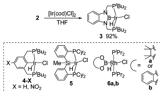
Scheme 2. Synthesis of PBP Iridium Complex 3 and Related Compounds 4 – 6
