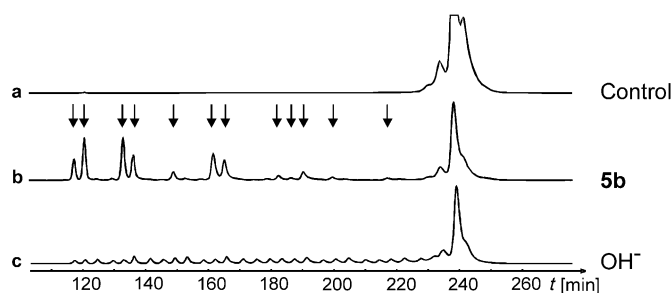
Fig. 2. Cleavage of substrate 7 induced by compound 5b . Control: Incubation of 7 in buffer for 16 h at 37° (lane a). RNA Cleavage shown in lane b was performed at 10 mM catalyst concentration in 50 mM Tris-HCl, 0.01% SDS buffer (pH 7.0). A base ladder of substrate 7 is depicted in lane c. RNA fragmentation was analyzed as described in the Exper. Part . Cleavage sites indicated by arrows are given in bold letters: Cy5-T 10 - CUAGCCGACUGCCGAUCUCGCUGACUGAC .
