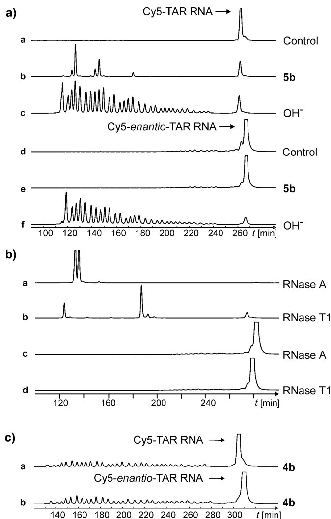
Fig. 7. Cy5-TAR RNA and Cy5-enantio-TAR RNA . a) The cleavage pattern produced by 5b (10 mM) with RNA 14 (lane b) is compared to that with enantio-RNA 15 (lane e). Controls contain only Cy5-labeled RNA substrates ( 14 : lane a; 15 : lane d). Base ladders are shown in lane c ( 14 ) and in lane f ( 15 ). b) Cy5-labeled TAR (lanes a and b) and enantio-TAR RNA (lanes c and d) were incubated with 10 ng RNase A and 1 unit RNase T1, respectively. c) Nonspecific base-cleavage pattern produced by 4b with TAR RNA 14 or enantio-TAR RNA 15 . Samples were run in parallel on denaturing PAGE.
