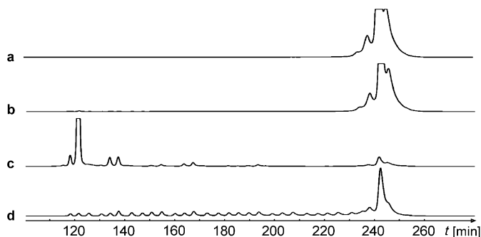
Fig. 3. Ultrafiltration to remove RNase contaminants. Lane a: Substrate 7 incubated for 20 h at 37°. Lane c: Substrate 7 after incubation with RNase A (1 ng/ml enzyme, 5 min, 37°). Lane b: The same solution of RNase A was subjected to ultrafiltration and incubated with 7 for 20 h at 37°. A base ladder of 7 is shown in lane d.
