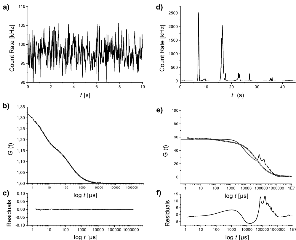
Fig. 8. Fluorescence-correlation spectroscopy (FCS) . Testing for aggregation of oligonucleotides by 4b and 5b . Diffusion of Cy5-labeled T 20 U molecules ( 17 ) through the confocal volume element was measured as fluorescence-intensity fluctuations. Count rate vs. time graphs are shown in a ) (buffer control) and d ) (250 \mu M 4b ), and the corresponding autocorrelation curves (— observed; ○ calculated) are shown in b ) (buffer control) and e ) (250 \mu M 4b ). The difference between observed and calculated data points is presented as residuals in c ) and f ). Upon addition of 5b up to 10 mM (not shown), the count rate vs. time graph shown in a ) did not change significantly. The constant diffusion times rule out aggregation phenomena.
