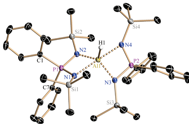
Figure 3. Molecular structure of 5 . Table 1 contains selected bond lengths [ \text{\AA} ] and angles [ ^\circ ]. Anisotropic displacement parameters are drawn at the 50% probability level. H atoms (except for those of Al1) and one THF solvent molecule are omitted for clarity.
