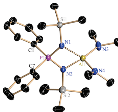
Figure 4. Molecular structure of 7 . Table 1 contains selected bond lengths [ \text{\AA} ] and angles [ ^\circ ]. Anisotropic displacement parameters are drawn at the 50% probability level. H atoms are omitted for clarity.
