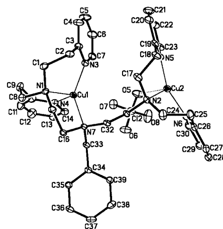
Fig. 1 ORTEP diagram of the cationic portion of complex 1 . Selected bond lengths (Å): Cu1...Cu2 5.432, Cu1-N1 2.135(3), Cu1-N3 1.979(3), Cu1-N4 2.024(3), Cu1-N7 2.106(3), Cu2-N2 2.252(3), Cu2-N5 1.927(3), Cu2-N6 1.925(3), Cu2-O5 2.551(3).
