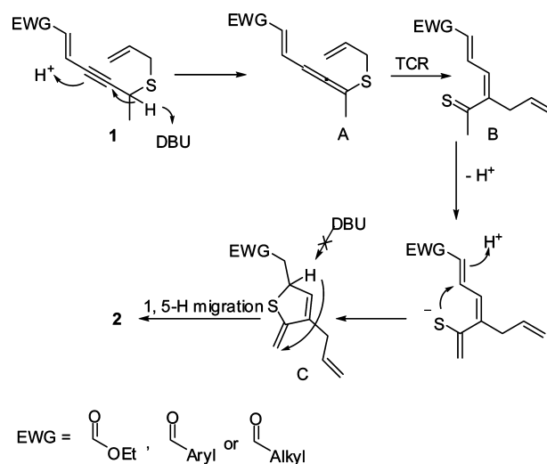
Scheme 3. Proposed Mechanism
