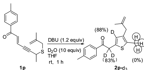
Scheme 4. Control Experiment
