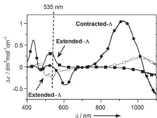
Figure 2. CD spectra of [\text{Co}(\text{H}_2\text{L1})(\text{CF}_3\text{SO}_3)(\text{H}_2\text{O})](\text{CF}_3\text{SO}_3)(\text{CHCl}_3) (■), [\text{Co}(\text{L1})] (●) and [\text{Co}(\text{H}_2\text{L1})(\text{CF}_3\text{SO}_3)(\text{H}_2\text{O})](\text{CF}_3\text{SO}_3)(\text{CHCl}_3) in the presence of five equivalents of \text{Bu}_4\text{NNO}_3 (○) in \text{CH}_3\text{CN}/\text{CHCl}_3 (1/9) at room temperature. [complex] = 2.5 \times 10^{-3} \text{ mol dm}^{-3} , 10 mm cuvette.
