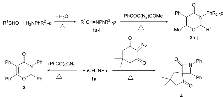
SCHEME 1 Reaction of \alpha -diazo- \beta -diketones and imines.
