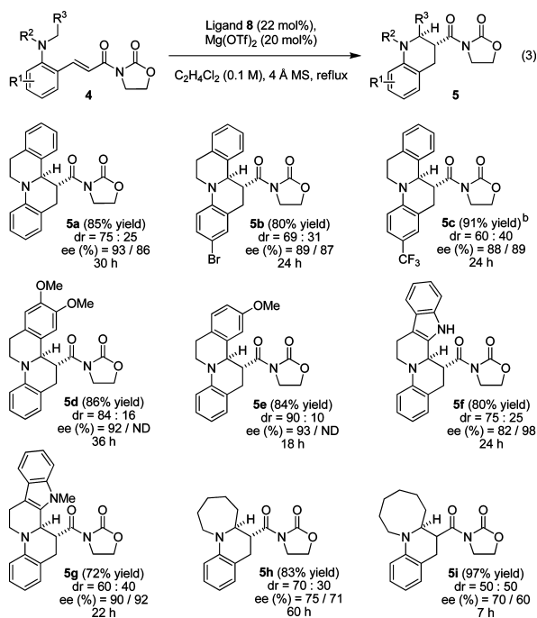
Chart 1. Scope of the Reaction a,b
