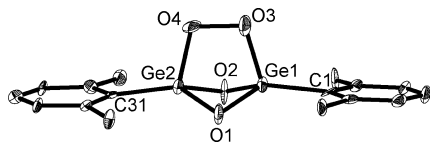
Figure 2. Thermal ellipsoid (50%) plot of 8 . H atoms and flanking rings are not shown. Selected bond distances (Å) and angles (deg): \text{Ge1-O1} , 1.792(5); \text{Ge2-O2} , 1.812 (5); \text{Ge1-O3} , 1.811(6); \text{Ge2-O4} , 1.825(5); \text{O3-O4} , 1.528(7); \text{Ge1-C1} , 1.911(6); \text{O1-Ge1-O2} , 87.1(2); \text{Ge1-O1-Ge2} , 84.2(2).
