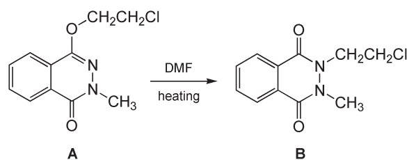
Figure 2. Isomerization of 4-(2-chloroethoxy)-2-methylphthalazin-1(2 H )-one ( A ) into 2-(2-chloroethyl)-2,3-dihydro-3-methylphthalazine-1,4-dione ( B ) [22].
