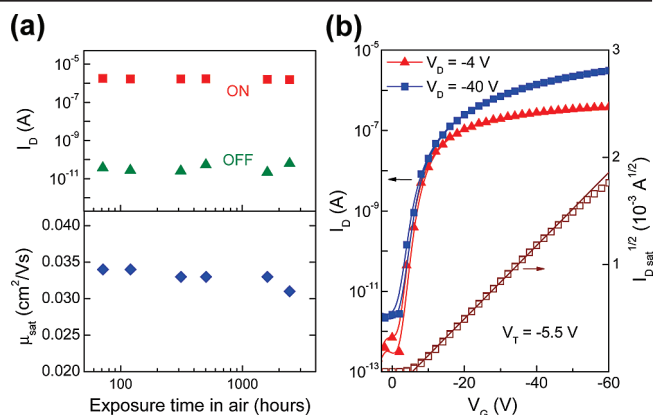
Figure 2. (a) (Top) Periodic ON and OFF currents and (bottom) charge carrier mobility measurements on ambient devices stored in air over a period of \sim 3 months. (b) Transfer characteristics of PIF8-TAA copolymer with L = 30 \mu\text{m} , W = 1000 \mu\text{m} , corresponding to a mobility of 3.8 \times 10^{-2} \text{ cm}^2/(\text{V s}) .
