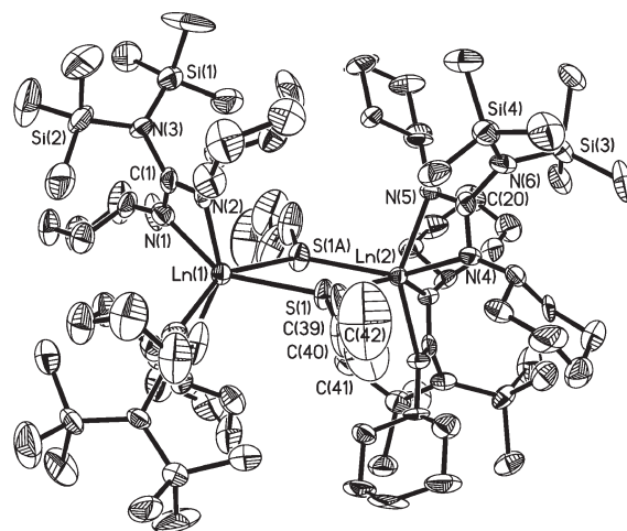
Figure 5. ORTEP diagram of \{[(\text{SiMe}_3)_2\text{NC}(\text{NCy})_2]_2\text{Ln}(\mu\text{-S}''\text{Bu})_2\}_2 [ \text{Ln} = \text{Y} ( 5-Y ), \text{Er} ( 5-Er ), \text{Yb} ( 5-Yb )] with the probability ellipsoids drawn at the 30% level. Hydrogen atoms are omitted for clarity.
