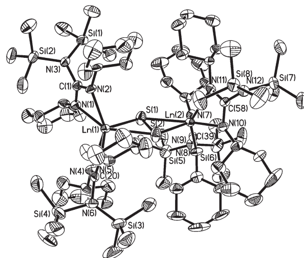
Figure 4. ORTEP diagram of \{[(\text{SiMe}_3)_2\text{NC}(\text{NCy})_2]_2\text{Ln}\}_2(\mu\text{-}\eta^2\text{-}\eta^2\text{-S}_2) [Ln = Er ( 4-Er ), Yb ( 4-Yb )] with the probability ellipsoids drawn at the 30% level. Hydrogen atoms are omitted for clarity. Selected bond lengths (Å) and angles (deg) for 4-Er : Er(1)–N(1) 2.303(8), Er(1)–N(2) 2.315(8), Er(1)–C(1) 2.712(10), N(1)–C(1) 1.309(12), N(2)–C(1) 1.498(13), Er(1)–S(1) 2.688(5), Er(1)–S(2) 2.667(7), Er(2)–S(1) 2.692(7), Er(2)–S(2) 2.667(5), S(1)–S(2) 2.120(6); N(1)–Er(1)–N(2) 57.7(3), N(2)–C(1)–N(1) 115.9(8), C(1)–N(1)–Er(1) 93.2(6), C(1)–N(2)–Er(1) 92.3(5), Er(1)–S(1)–Er(2) 132.2(2), Er(1)–S(2)–Er(2) 134.4(2), S(1)–Er(1)–S(2) 46.6(1), S(1)–Er(2)–S(2) 46.6(1). For 4-Yb : Yb(1)–N(1) 2.306(6), Yb(1)–N(2) 2.299(6), Yb(1)–C(1) 2.721(8), N(1)–C(1) 1.290(10), N(2)–C(1) 1.320(10), Yb(1)–S(1) 2.671(3), Yb(1)–S(2) 2.652(3), Yb(2)–S(1) 2.670(3), Yb(2)–S(2) 2.645(3), S(1)–S(2) 2.114(3); N(1)–Yb(1)–N(2) 57.0(2), N(2)–C(1)–N(1) 114.7(7), C(1)–N(1)–Yb(1) 94.1(5), C(1)–N(2)–Yb(1) 93.6(5), Yb(1)–S(1)–Yb(2) 132.0(1), Yb(1)–S(2)–Yb(2) 134.2(1), S(1)–Yb(1)–S(2) 46.8(1), S(1)–Yb(2)–S(2) 46.9(1).
