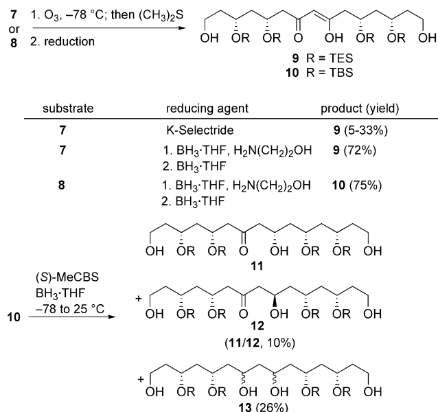
Scheme 3. Exploration of path A.
