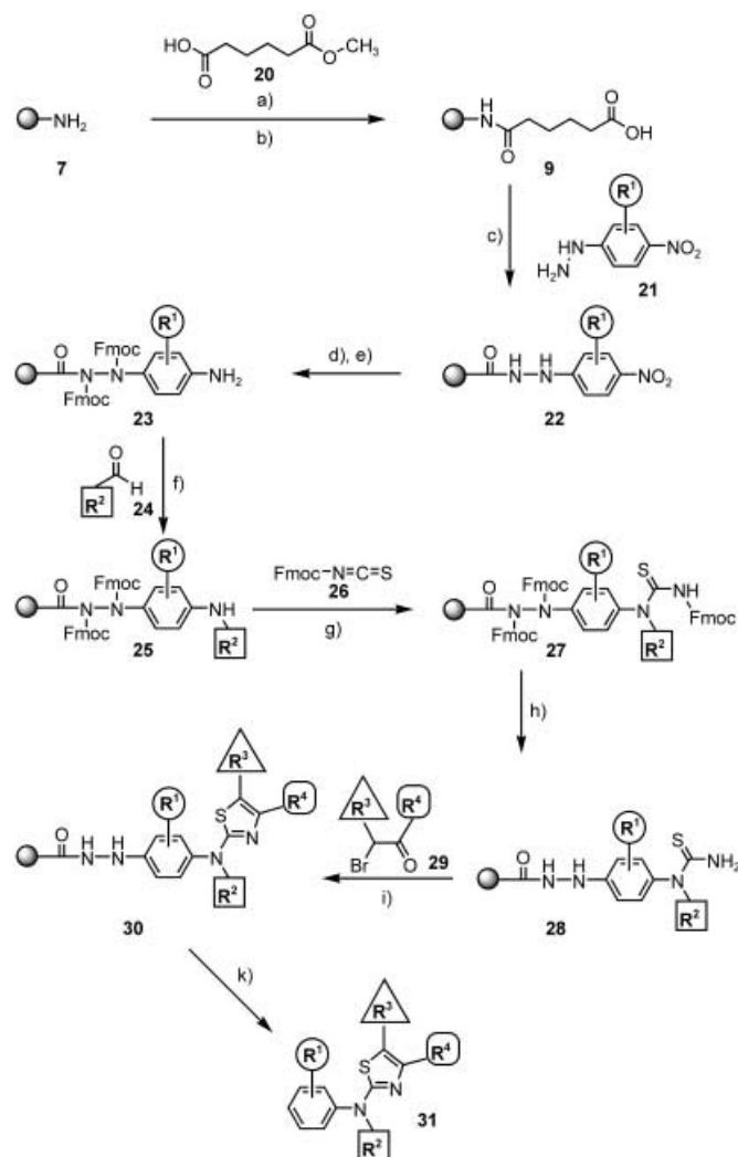
Scheme 4. Traceless solid-phase synthesis of 2-aminothiazoles 31 . a) 3 equiv adipic monomethyl ester ( 20V ), 3 equiv DIC, 3 equiv HOBt, 3 equiv NEt 3 , CH 2 Cl 2 , RT, 18 h; b) THF/1% LiOH 1:1, RT, 24 h; c) 3 equiv nitrophenylhydrazine ( 21 ), 3 equiv DIC, 3 equiv HOBt, 3 equiv NEt 3 , CH 2 Cl 2 , RT, 18 h; d) 10 equiv Fmoc-Cl, pyridine, CH 2 Cl 2 , 15 h; e) 2 M SnCl 2 × 2 H 2 O, DMF, RT, 18 h; f) 10 equiv aldehyde 24 , THF, HOAc, RT, 1 h, wash, then 10 equiv NaCNBH 3 , THF/HOAc, RT, 15 h; g) 3 equiv Fmoc-NCS 26 , CH 2 Cl 2 , pyridine, RT, 15 h; h) DMF/piperidine 4:1, RT, 2 × 5 min; i) 0.1 M solution of 29 in dioxane, RT, 2 × 3 h; k) 0.5 equiv [Cu(OAc) 2 ], n -propylamine, O 2 , RT, 2 h, then solid-phase extraction.
