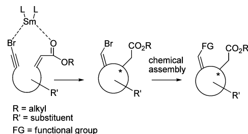
Figure 1. Basic concept for \text{SmI}_2 -promoted cyclization.
