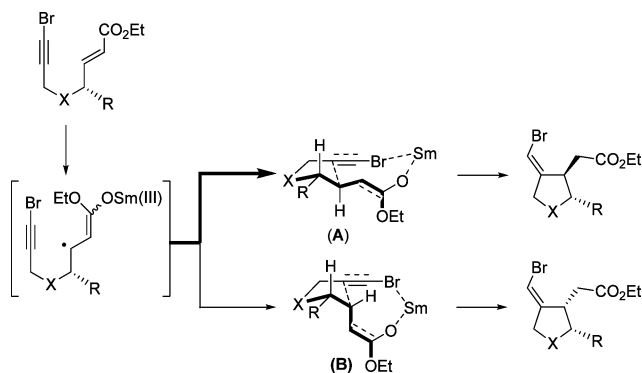
Figure 2. Plausible \text{SmI}_2 -mediated coupling of ( E )- \alpha,\beta -unsaturated esters.
