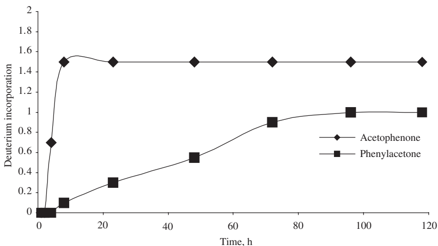
Figure 3. Variation of incorporation over time (2:1 substrate/catalyst) for ortho -deuteration of acetophenone and phenylacetone with complex 3a
