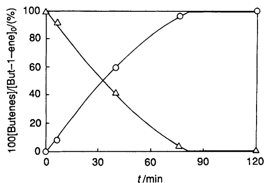
Figure 2. Time course of the photoisomerization of but-1-ene ( \Delta ) to trans -but-2-ene ( \circ ) with [\text{MoH}_4(\text{dppe})_2]
