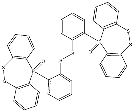
FIGURE 2 Representation of structure of compound reported in literature [15] as [OPS 3 ] 2 .
