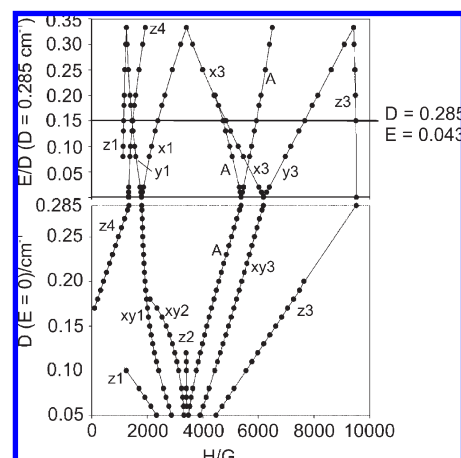
FIGURE 14. Simulation of the field dependence of the most intense axial transitions of a quartet system with D values between 0.05 and 0.285 \text{cm}^{-1} and E/D between 0 and 0.35. The values |D/hc| = 0.285 and |E/hc| = 0.043 \text{ cm}^{-1} of 5f are marked.
