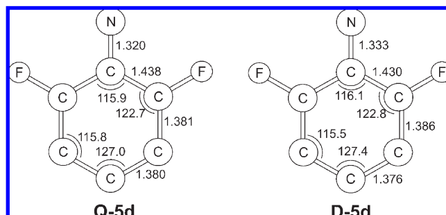
FIGURE 15. Geometries of the ^4A_2 state of Q-5d and the ^2A_2 state of D-5d from the UB3LYP/6-311G(d,p) level of theory. Both states show C_{2v} symmetry and the bond lengths and angles, as well as the calculated IR spectra, are quite similar.
