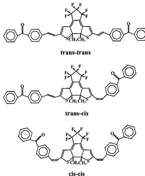
Figure 3. Structure formula of the three cis-trans isomers of bpe-BMTFP.
