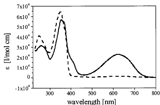
Figure 2. Absorption spectra of the closed isomer (thick solid line) and the open isomer (thick dashed line) of bpe-BMTFP in a 1.1 \cdot 10^{-5} mol/L \text{CH}_2\text{Cl}_2 solution.
