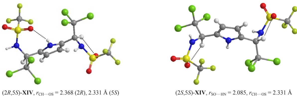
Fig. 2. Molecular structures of (2 S ,5 S )- and (2 R ,5 S )-diastereoisomers of 2,5-bis[2,2,2-trichloro-1-(trifluoromethylsulfonfylamino)-ethyl]pyrrole ( XIV ) according to B3LYP/6-311G( d,p ) calculations. Intramolecular hydrogen bonds are shown with dashed lines.
