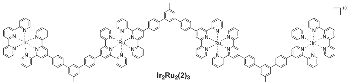
Figure 10. Structural formula of \text{Ir}_2\text{Ru}_2(2)_3 .
