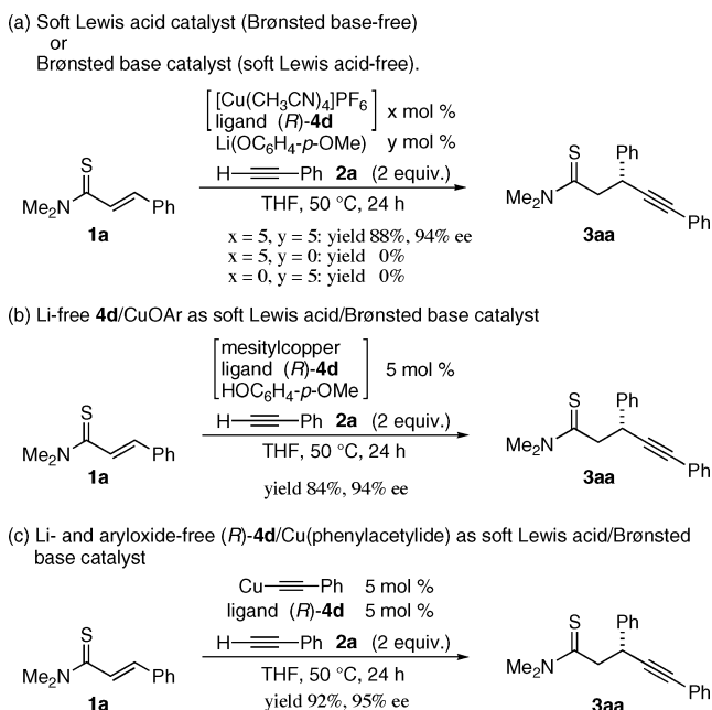
Scheme 2. Control Experiments
