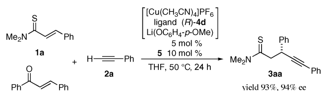
Scheme 1. Chemoselective Activation of Thioamide
