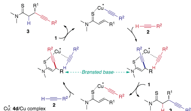
Figure 1. Plausible catalytic cycle with ( R )- 4d /Cu alkynylid catalyst.
