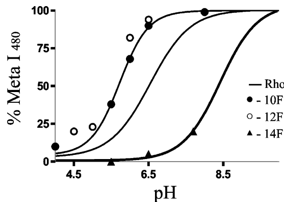
Figure 4. pH dependence of the Meta I ↔ Meta II equilibrium in native rhodopsin (solid line without data points) and the three fluoro analogues (symbolized as indicated) measured at 10 °C (283 K). The Rho and 14-F data could be fitted with a regular Henderson–Hasselbalch function. The 10-F and the 12-F data show a much steeper transition, which renders determination of a single \text{pK}_a value not reliable.
