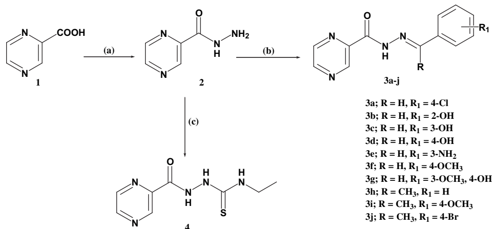
Scheme 1. Reagents and conditions; a) (i) \text{Et}_3\text{N} , \text{ClCOOEt} , \text{MeOH} , (ii) \text{NH}_2\text{NH}_2 \cdot \text{H}_2\text{O} b) Aldehyde or Ketone, \text{EtOH} , reflux c) \text{EtNCS} , \text{EtOH} , reflux.
