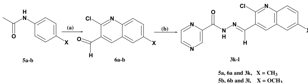
Scheme 2. Reagents and conditions; a) \text{POCl}_3 , \text{DMF} b) \text{EtOH} , reflux.
