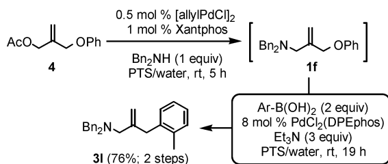
Scheme 4. Proposed Mechanism
