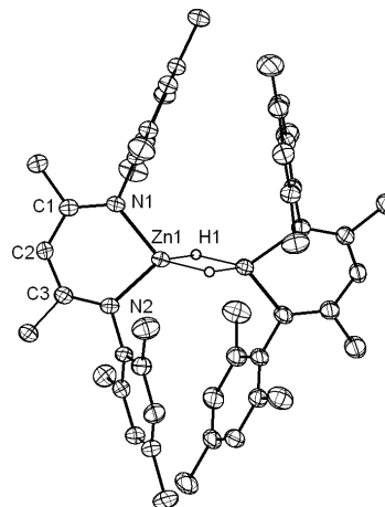
Fig. 2. Molecular structure of the P2 / n polymorph of 1 in the crystal ( 1b ). The molecule has a crystallographically imposed C 2 axis.
