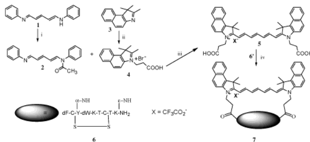
Scheme 1. Synthesis of NIR Macrocyclic Optical Scaffold a
