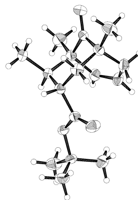
Fig. 2 ORTEP drawing of \alpha -7-endo,8- exo - 4b showing the thermal ellipsoids at the 30% probability level.
