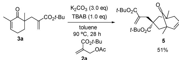
Scheme 2 Intramolecular Michael reaction of 3a in the presence of acrylate 2a .
