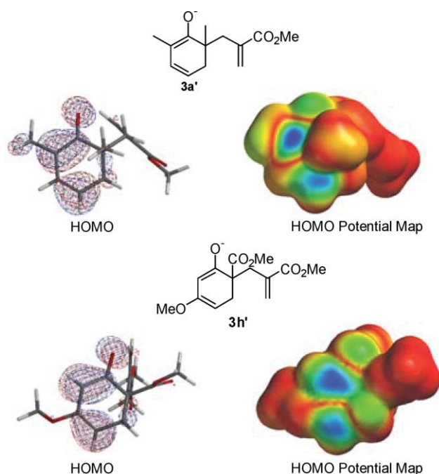
Fig. 4 HOMOs and HOMO potential maps of the enolates of 3a' and h' by B3LYP/6–31G* calculations.
