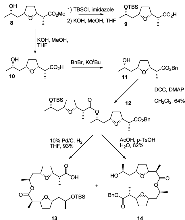
Scheme 2. Completion of the Synthesis of All-(–)-nonactin
