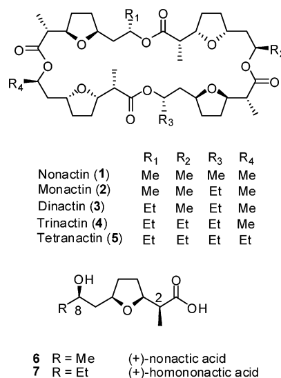
Figure 1. Structures of nonactin and the naturally occurring macrotetrolides.
