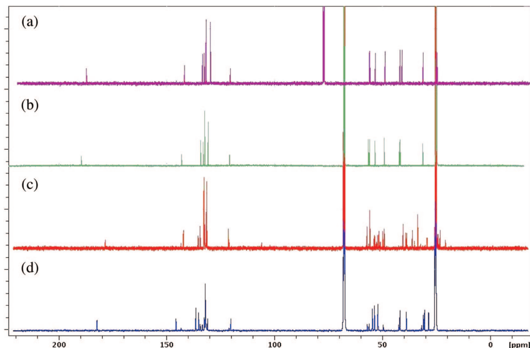
FIGURE 3. ^{13}\text{C} NMR spectra of compound 4 dissolved in (a) \text{CDCl}_3 , (b) 1:1 \text{D}_2\text{O}/\text{THF}-d_8 , (c) 1:6 \text{DCl} (1 N in \text{D}_2\text{O} )/ \text{THF}-d_8 , and (d) 1:6 \text{NaOD} (1 N in \text{D}_2\text{O} )/ \text{THF}-d_8 .
