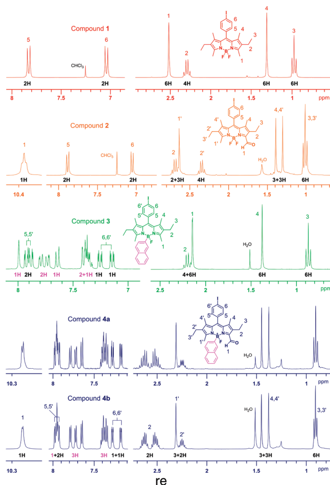
Figure 2. ^1\text{H} NMR spectra of 1 , 2 ( \text{CDCl}_3 , RT), 3 , 4a , and 4b ( \text{CD}_2\text{Cl}_2 , RT).
