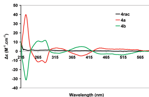
Figure 3. CD spectra of 4 rac , 4a , and 4b in \text{CH}_2\text{Cl}_2 at RT.
