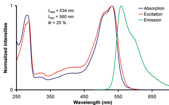
Figure 4. Absorption (blue line), emission (green line), and excitation (red line) spectra of 4a , in \text{CHCl}_3 at RT and at a concentration of ca. 1 \times 10^{-6} M.
