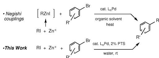
Scheme 1. Zn-Mediated, Pd-Catalyzed Cross-Couplings with Aryl Bromides
