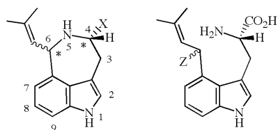
(4 S , 6 R )- 1a : X = CO 2 H (4 S , 6 S )- 1b : X = CO 2 H (±)- 1c : X = H
