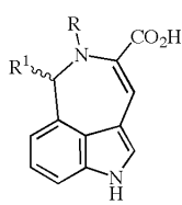
3a (R = H; R' = Me) 3b (R = H; R' = i -Pr) 3c (R = H; R' = i -Bu) 3d (R = PhCO; R' = H)
