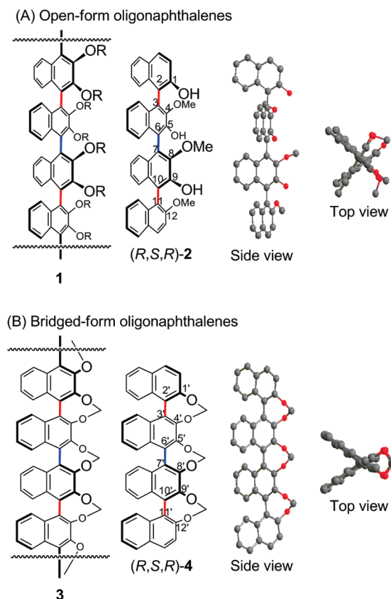
Figure 1. Optimized geometries obtained by DFT calculations at the B3LYP/6-31G(d) level for the (A) open- and (B) bridged-form oligonaphthalenes; Red axes denote R configuration and blue axes denote S configuration.
