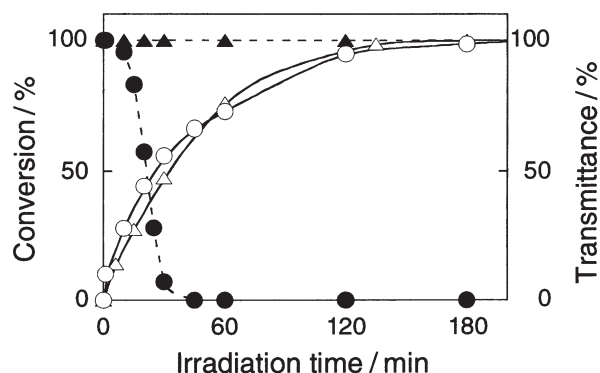
Figure 1. Conversions of 1 and 2 and transmittances of their solutions versus irradiation time: [surfactant] = 1.0 \times 10^{-2} M; circle, 1 ; triangle, 2 ; open symbols, conversion; closed symbols, transmittance at 500 nm.
