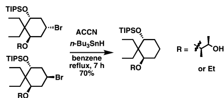
Scheme 2. Confirmation of the Relative and Absolute Stereochemistry of the Minor Product in Table 1, Entry 5, and Table 2, Entry 3
