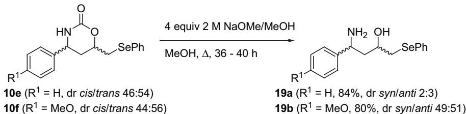
Scheme 6.
