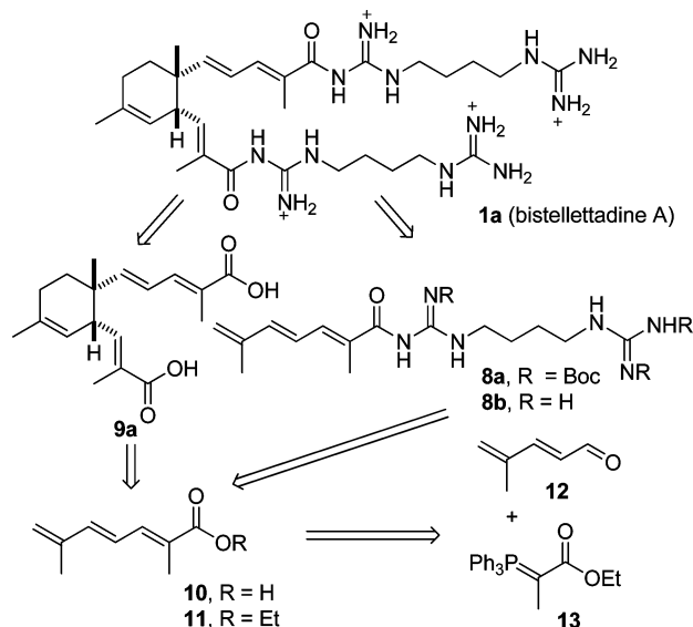
Scheme 2. Retrosynthesis of ( \pm )-Bistellettadine A ( 1a )
