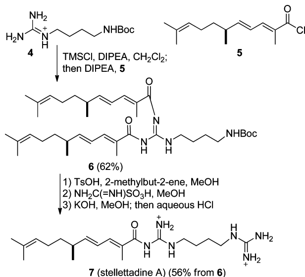
Scheme 1. Mori's Synthesis of Stellettadine A ( 7 )
