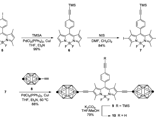
Scheme 1. Synthesis of Axle 10
