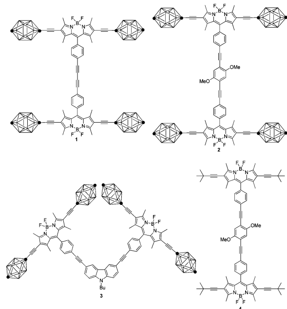
Figure 1. Structure of BODIPY-based nanocars 1–3 and analogue 4 . Every vertex of the carborane wheel is BH except the darkened sites, where the outer (para) is CH and the inner (ipso) is alkynyl-substituted C.
