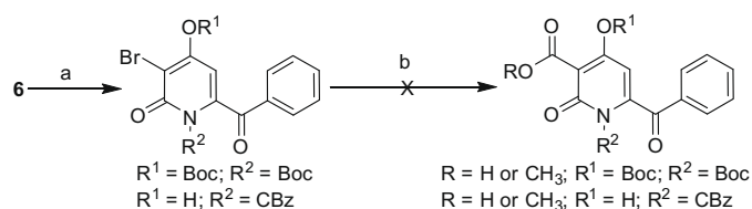
Scheme 3. Reagents and conditions: (a) Boc anhydride, \text{DCM} , \text{TEA} , 0^\circ\text{C} to rt, 6 h, 90% or \text{CBzCl} , \text{TEA} , \text{DCM} , 0^\circ\text{C} to rt, 3 h; (b) bis(benzonitrile)palladium(II) chloride, \text{dppf} , \text{TEA} , \text{MeOH} , \text{CO} , 300 psi, 120 °C, 12 h or \text{BuLi} , \text{THF} , -78^\circ\text{C} , 1 h, then \text{CO}_2 .
