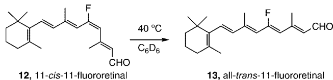
FIGURE 6. Thermal rearrangement of 11- cis -11-fluororetinol 12 .
