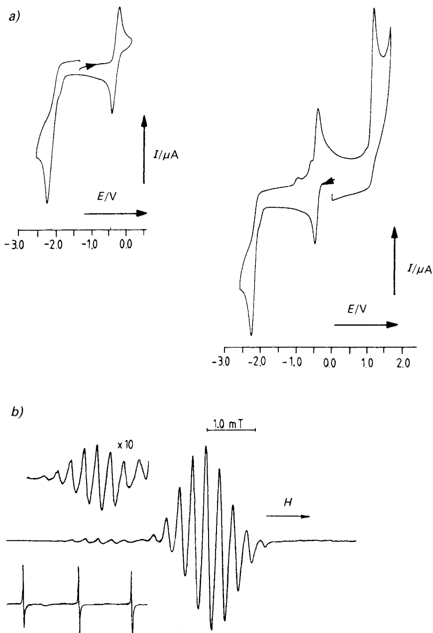
Fig. 1. a) Cyclic voltammograms of 8 in DME/0.1M \text{Bu}_4\text{NClO}_4 vs. SCE at glassy carbon. T = 25^\circ , v = 0.05 \text{ Vs}^{-1} , E_{\text{pc}} = -2.22 \text{ V} (irreversible), E_{1/2}^{+0} = -0.45 \text{ V} , \Delta E_{1/2} = 78 \text{ mV} (reversible), E_{\text{pa}} = 1.22 \text{ V} (irreversible). b) EPR spectrum of \mathbf{8}^{+\bullet} (air oxidation, \text{CHCl}_3/\text{DMF} 1:1, 25^\circ ). \langle g \rangle = 1.9866 , a(10^4 \text{ H}) = 0.325 \text{ mT} , a(^{53}\text{Cr}) = 1.78 \text{ mT} .
