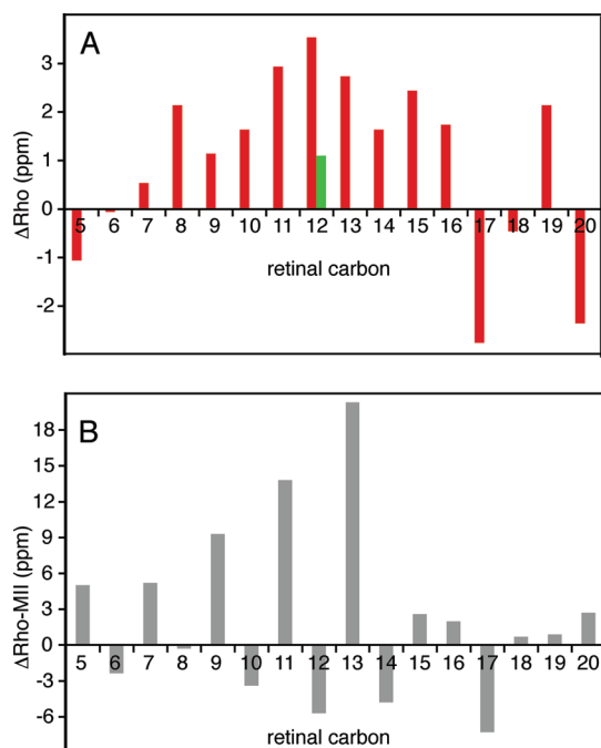
Figure 3. Comparison of retinal 13 C chemical shifts in rhodopsin with an 11- cis retinal PSB model compound and with Meta II. (A) Differences Δ(Rho) are plotted between the retinal chemical shifts for C5–C20 carbons in rhodopsin and in the N -(11- cis -retinylidene)- n -propyliminium trifluoroacetate model compound in solution (red). 43 The measurement of the 13 C12 chemical shift in the E181Q mutant of rhodopsin is also shown (green bar). (B) Differences Δ(Rho–MII) are plotted between the retinal chemical shifts for C5–C20 plotted in rhodopsin and Meta II. All chemical shifts are externally referenced to neat TMS.
